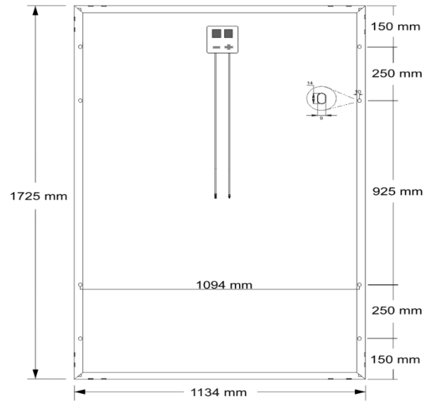
Mechanical Diagrams
