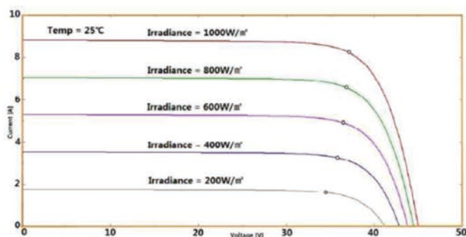
IV-Curves
